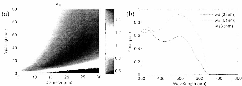
Fig. 4. (a) Absorption enhancement as a function of MNP diameter and spacing between neighboring MNPs. (b) Absorption spectra for a solar cell (33nm) with (w) and without (wo) 24nm diameter MNPs and for a solar cell (61nm) without MNPs.
