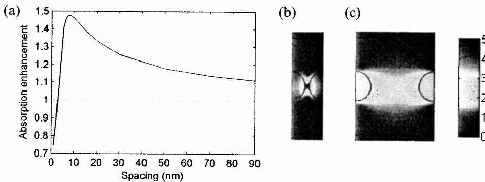
Fig. 2. (a) Spacing dependence of Absorption enhancement. Depictions of the electric field enhancement with spacings (b) 2nm and (c) 16nm.
