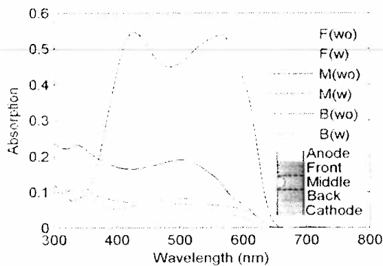
Fig. 3. Absorption spectra with MNPs (w) and without MNPs (wo) in front (F), middle (M) and back (B) layers when MNPs are embedded in the middle layer with 8nm spacing.
