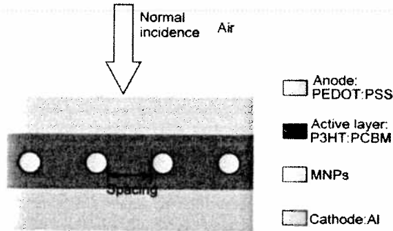
Fig. 1. Schematic picture of OSCs under investigations
